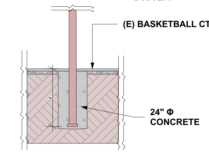
BASKETBALL POST
